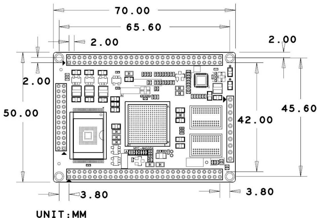
MYC-C335X-V4 Dimension Chart
