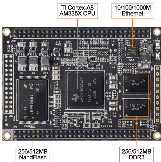
MYC-C335X-V4 Top-view
