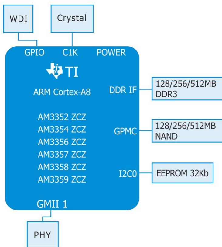
MYC-C335X-V4 Function Block Diagram
