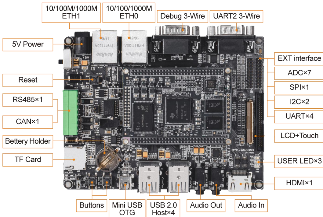
MYD-C335X-V4 Development Board
