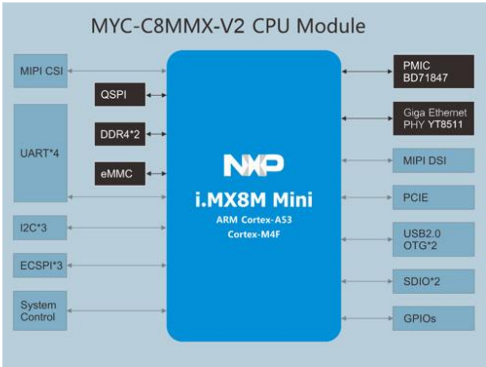
MYC-C8MMX-V2 CPU Module Function Block Diagram
