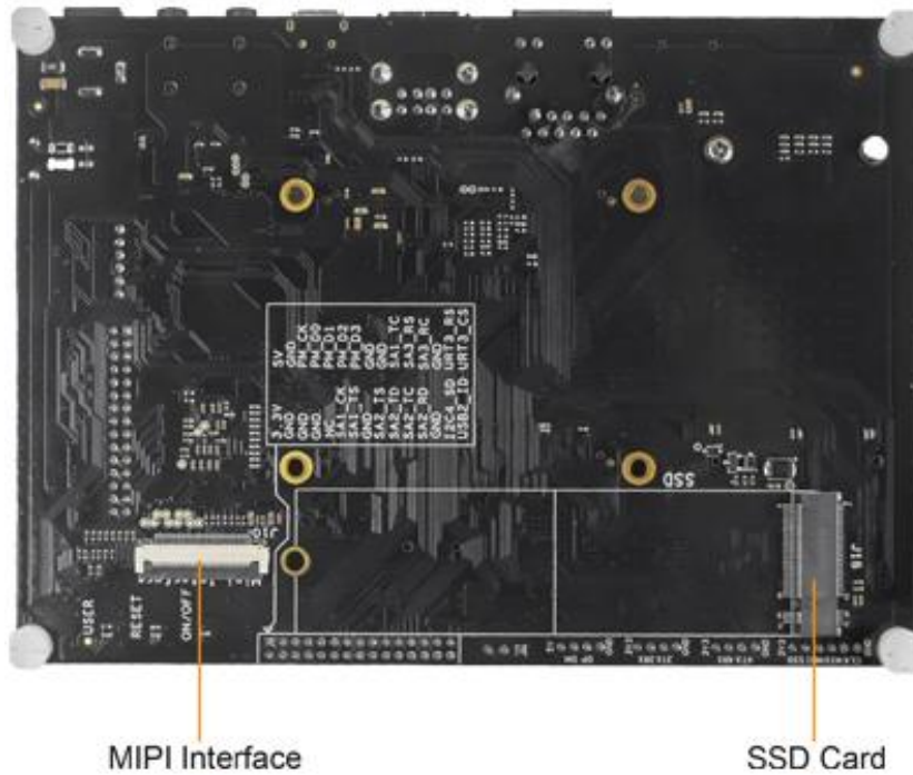
MYD-C8MMX-V2 Development Board Bottom-view
