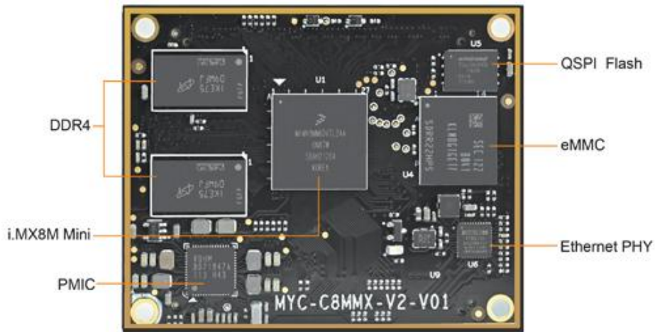
MYC-C8MMX-V2 CPU Module Top-View
