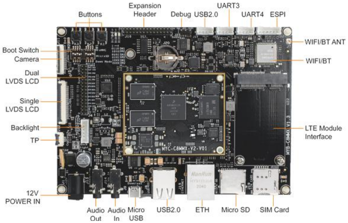
MYD-C8MMX-V2 Development Board Top-view
