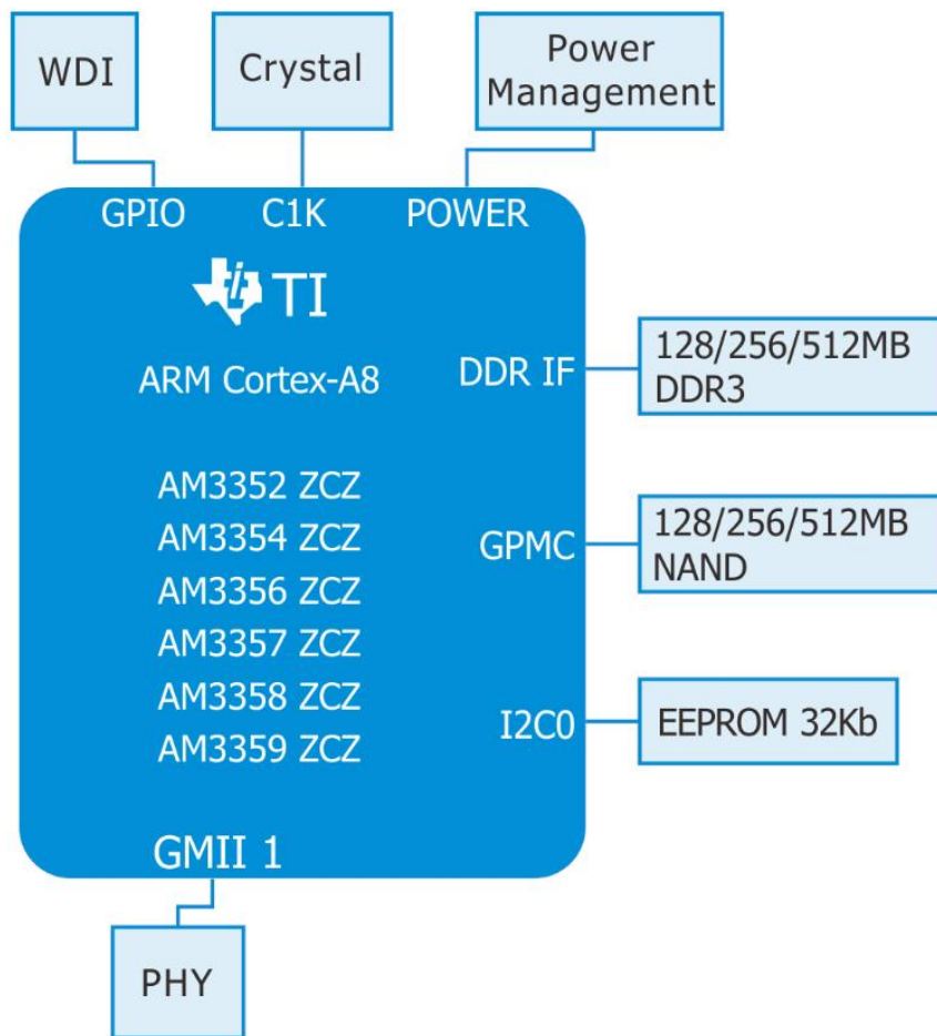
Function Block Diagram of MYC-J335X-V2
