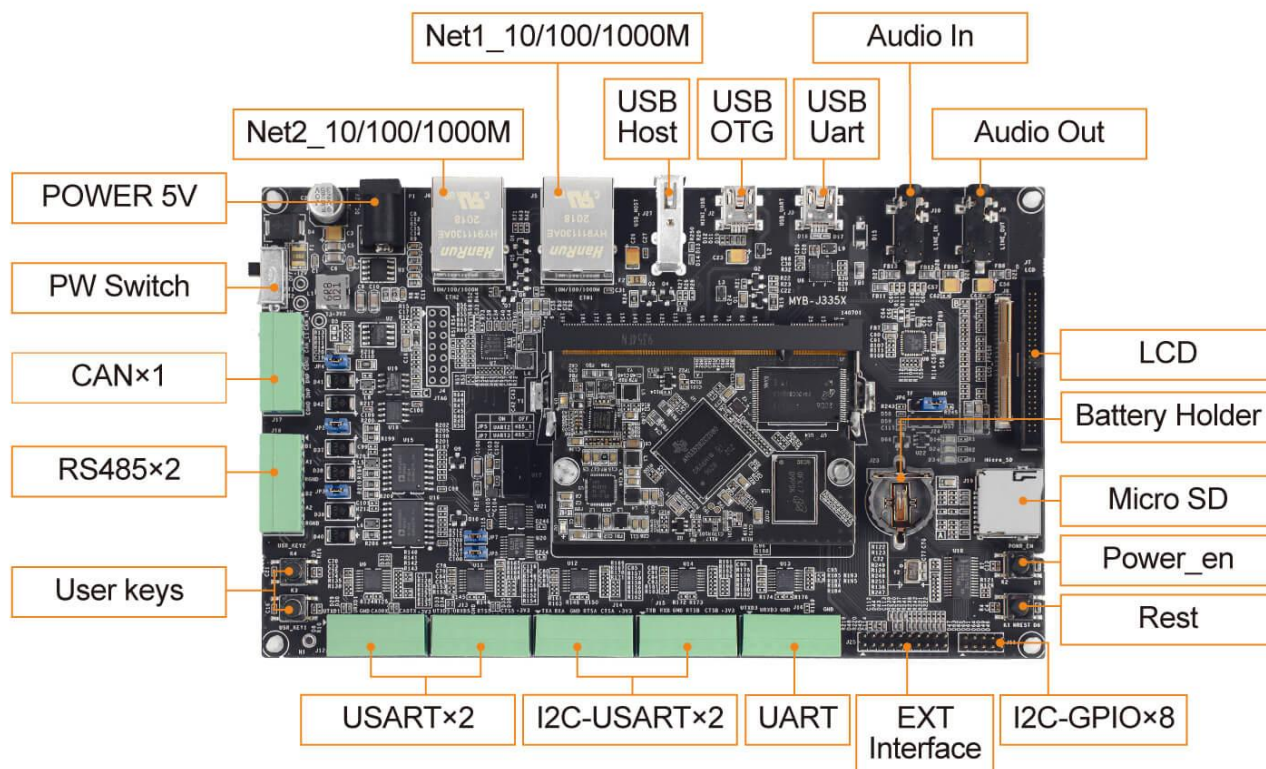
MYD-J335X-V2 Development Board
