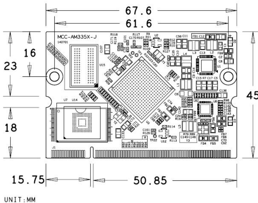
Dimensions of MYC-J335X-V2
