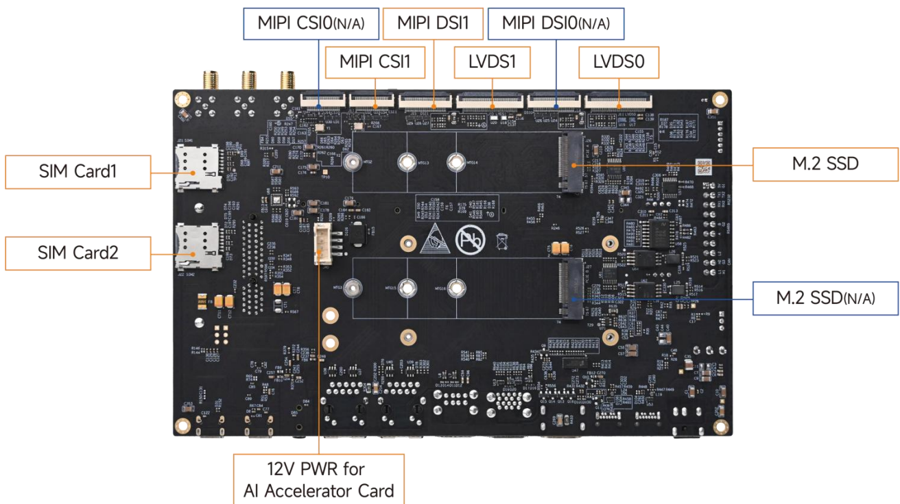
MYD-JMX95X Development Board (Bottom-view)
