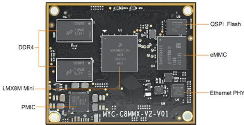
MYC-C8MMX-V2 Top-view
