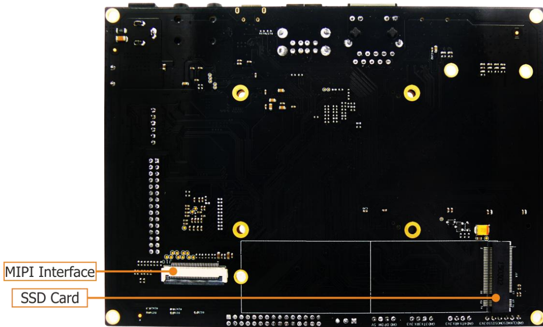
MYD-C8MMX-V2 Development Board Bottom-view
