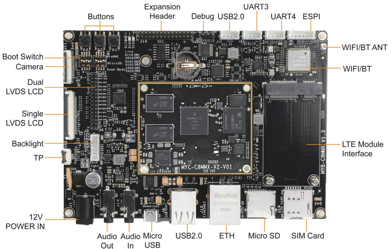
MYD-C8MMX-V2 Development Board Top-view
