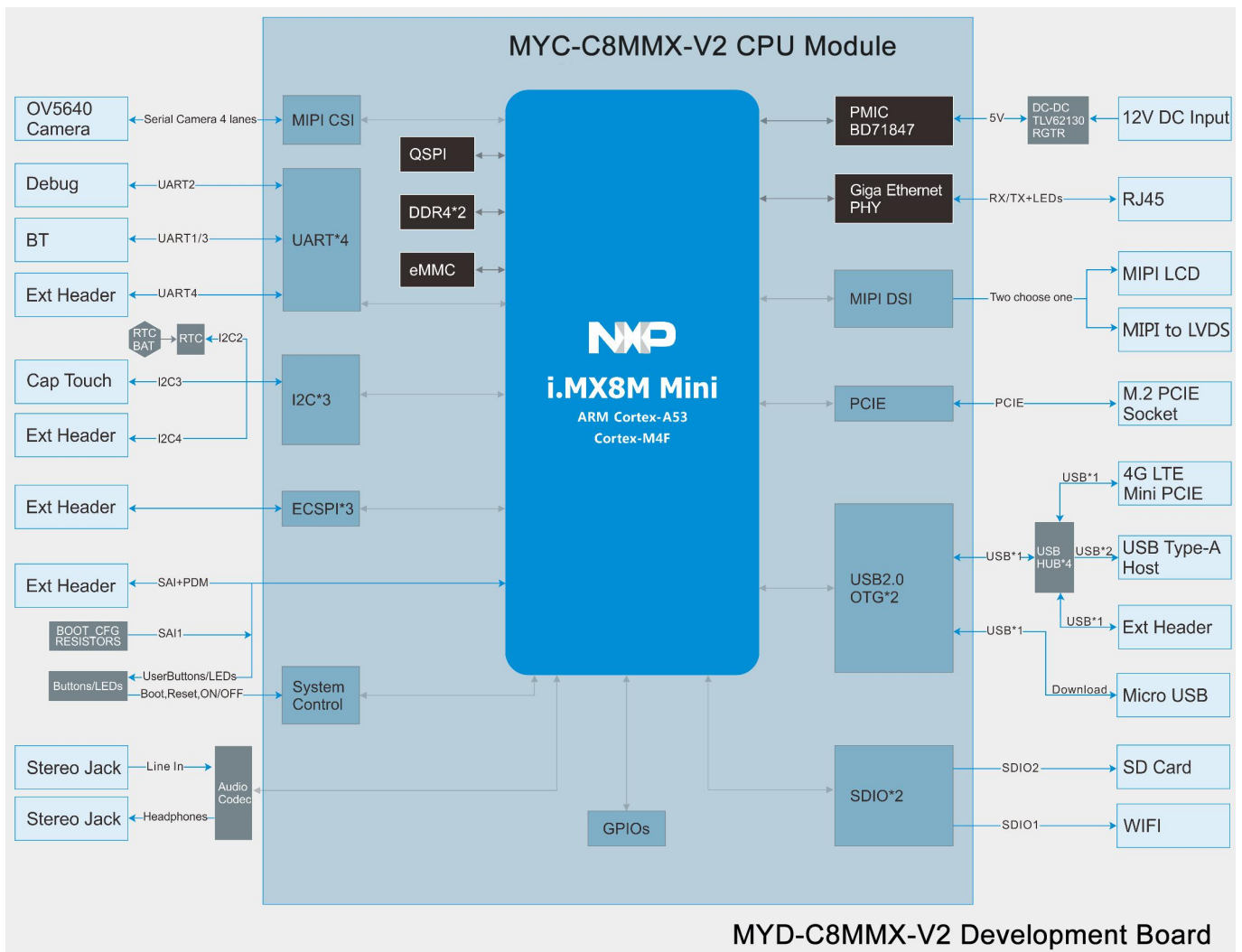
MYD-C8MMX-V2 Development Board Function Block Diagram
