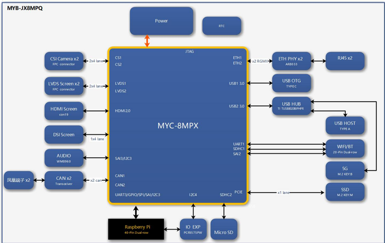
MYD-JX8MPQ Development Board Function Block Diagram
