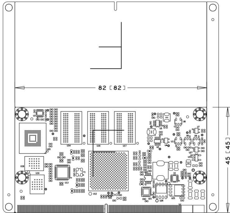
MYC-JX8MPQ Dimensions Chart
