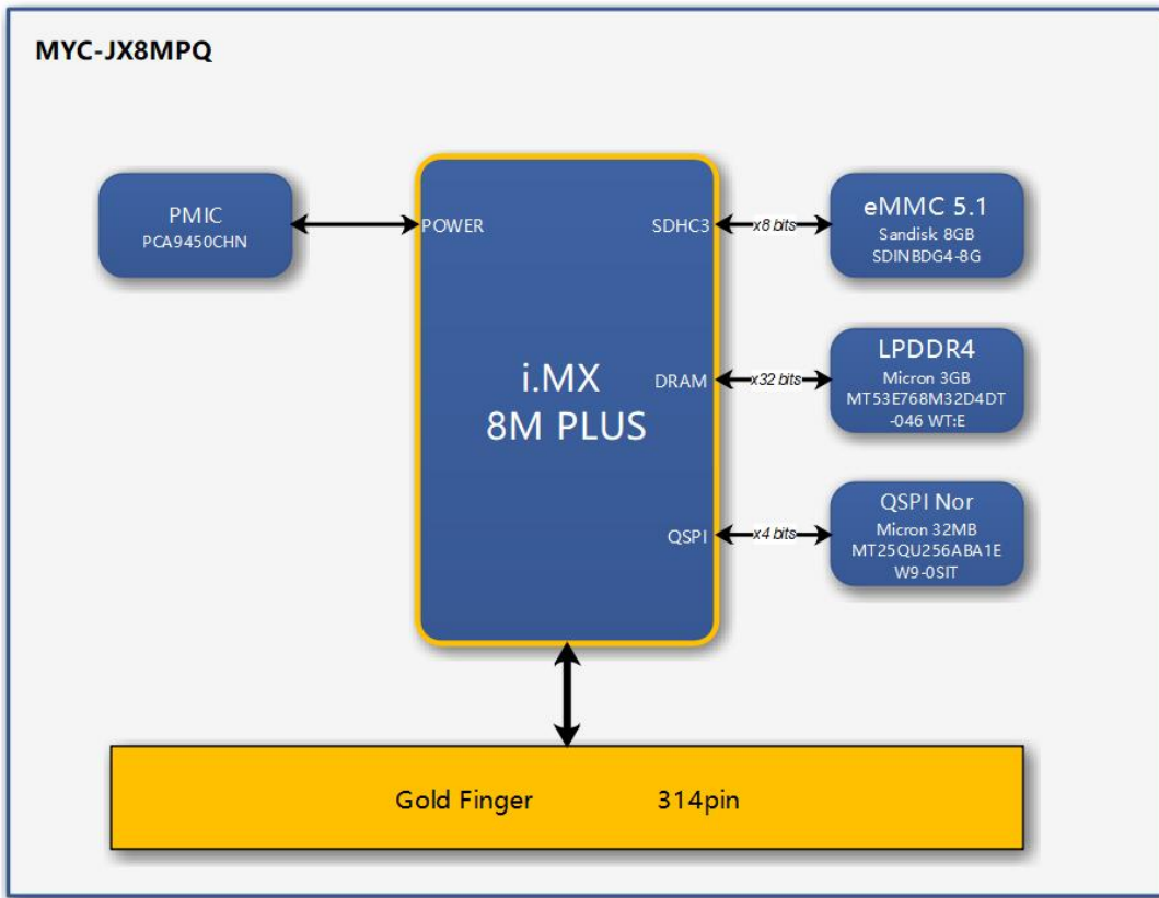
MYC-JX8MPQ Function Block Diagram
