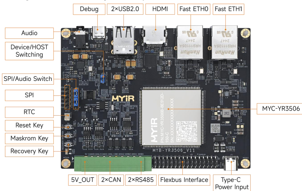
MYD-YR3506 Development Board (Top view)
