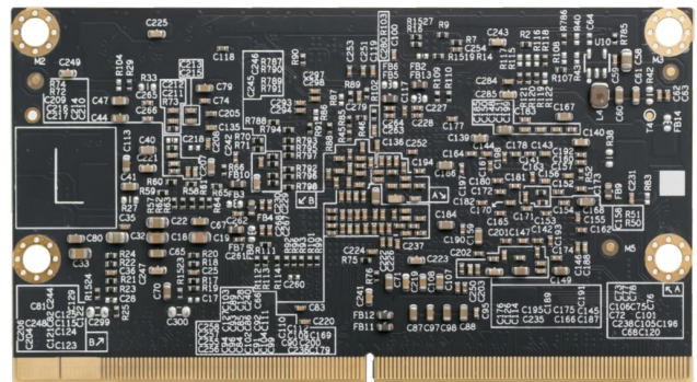
MYC-JD9360 CPU Module (Bottom-view)
