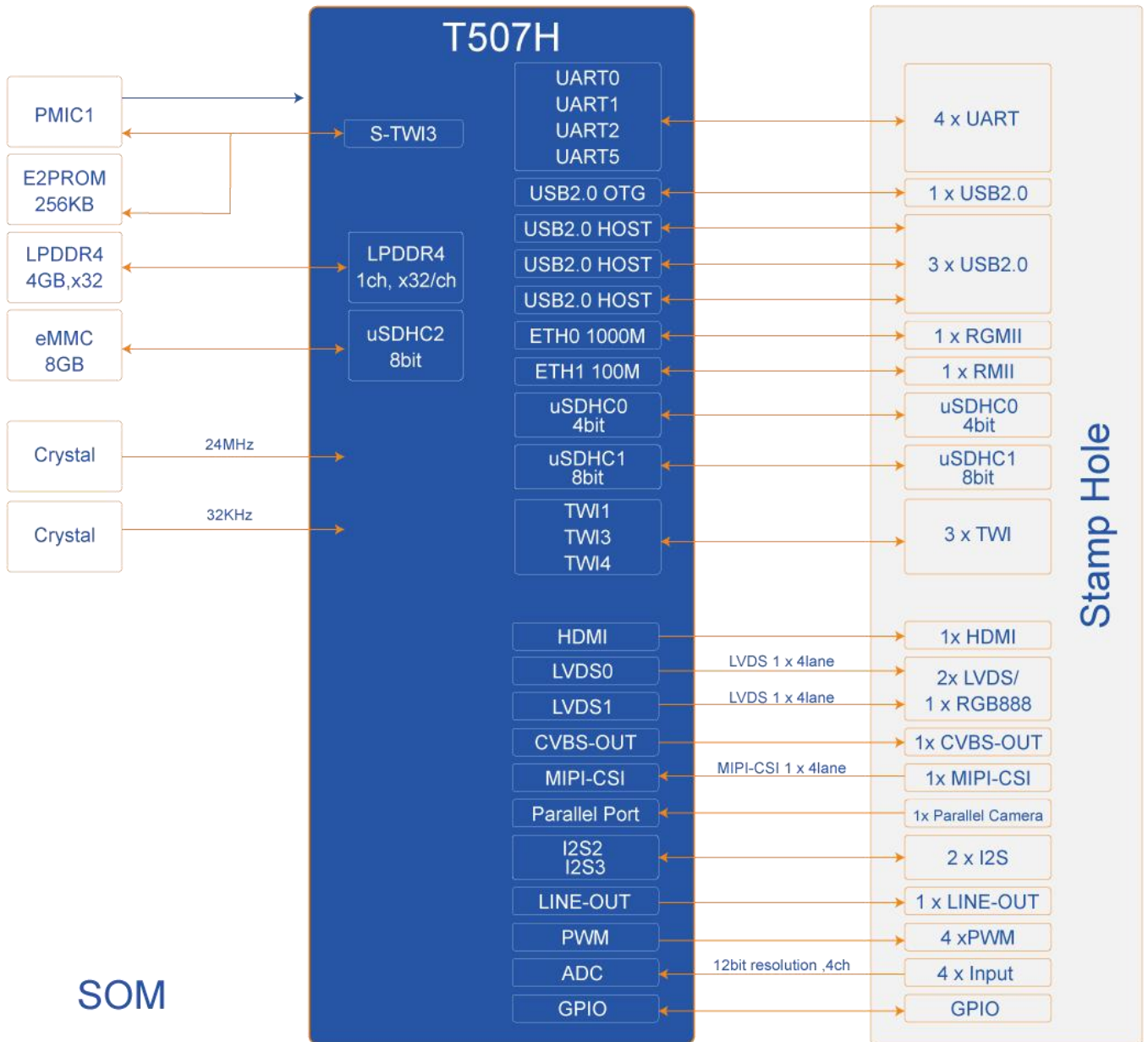
MYC-YT507H CPU Module Block Diagram
