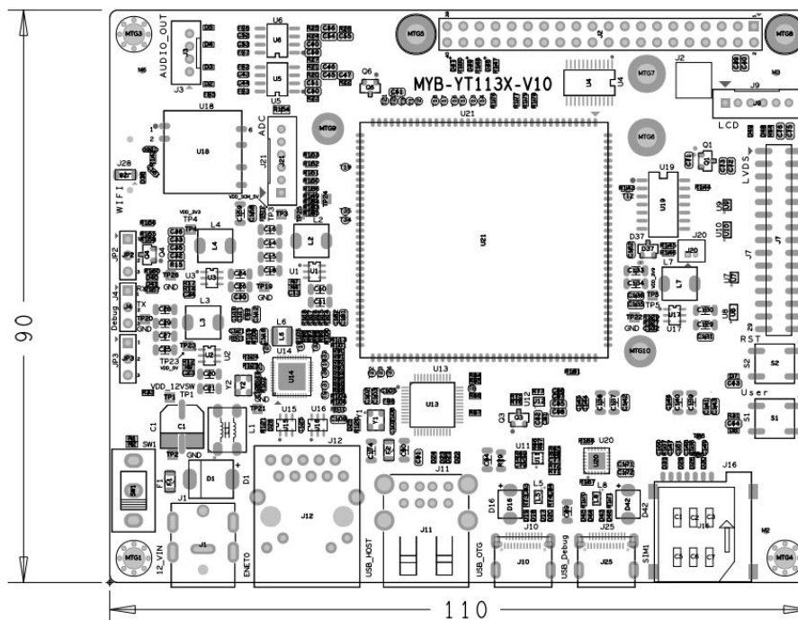
MYB-YT113X-V10 Dimensions Chart (Unit: mm)
