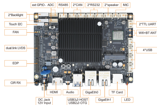
MYD-LT527-SX Top-view
