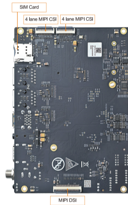
MYD-LT527-SX Bottom-view
