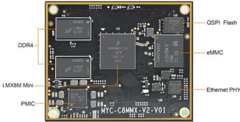
MYC-C8MMX-V2 CPU Module Top-view
