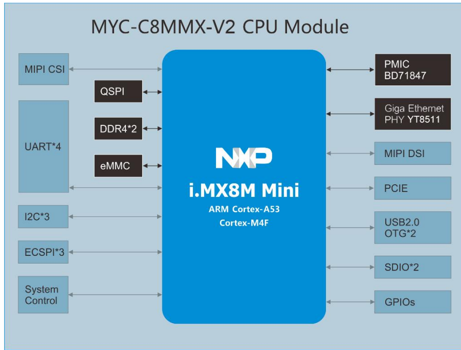
MYC-C8MMX-V2 CPU Module Function Block Diagram
