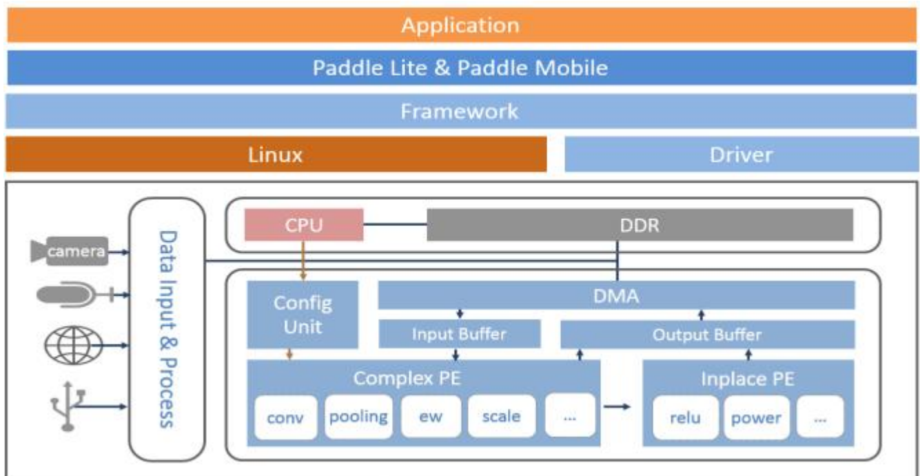
Software Architecture of FZ5 EdgeBoard AI Box
