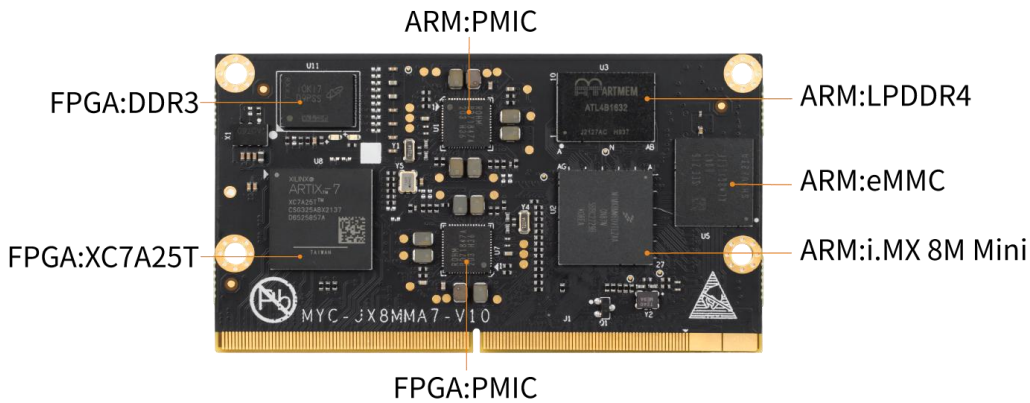
MYC-JX8MMA7 CPU Module Top-view
