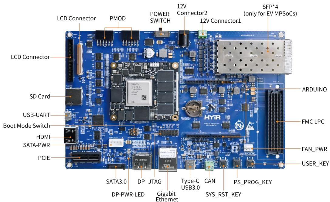
MYD-CZU3EG/4EV/5EV-V2 Development Board
