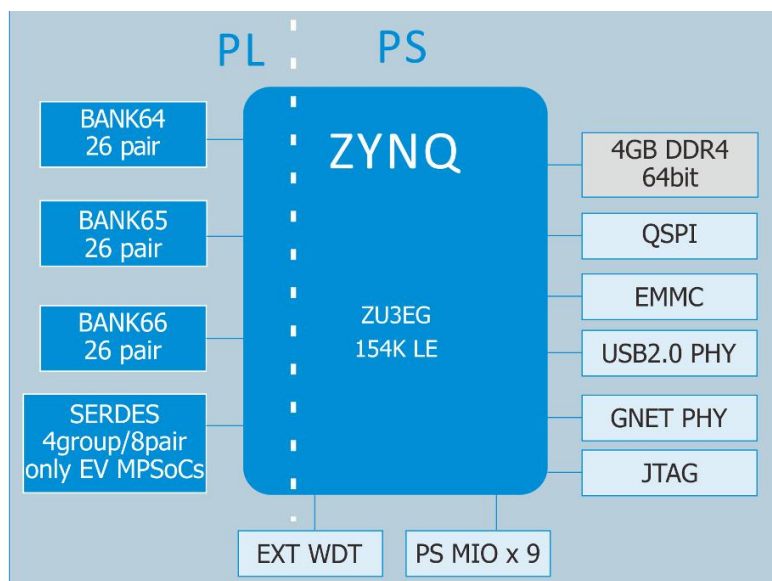
Function Block Diagram of MYC-CZU3EG/4EV/5EV-V2 CPU Module
